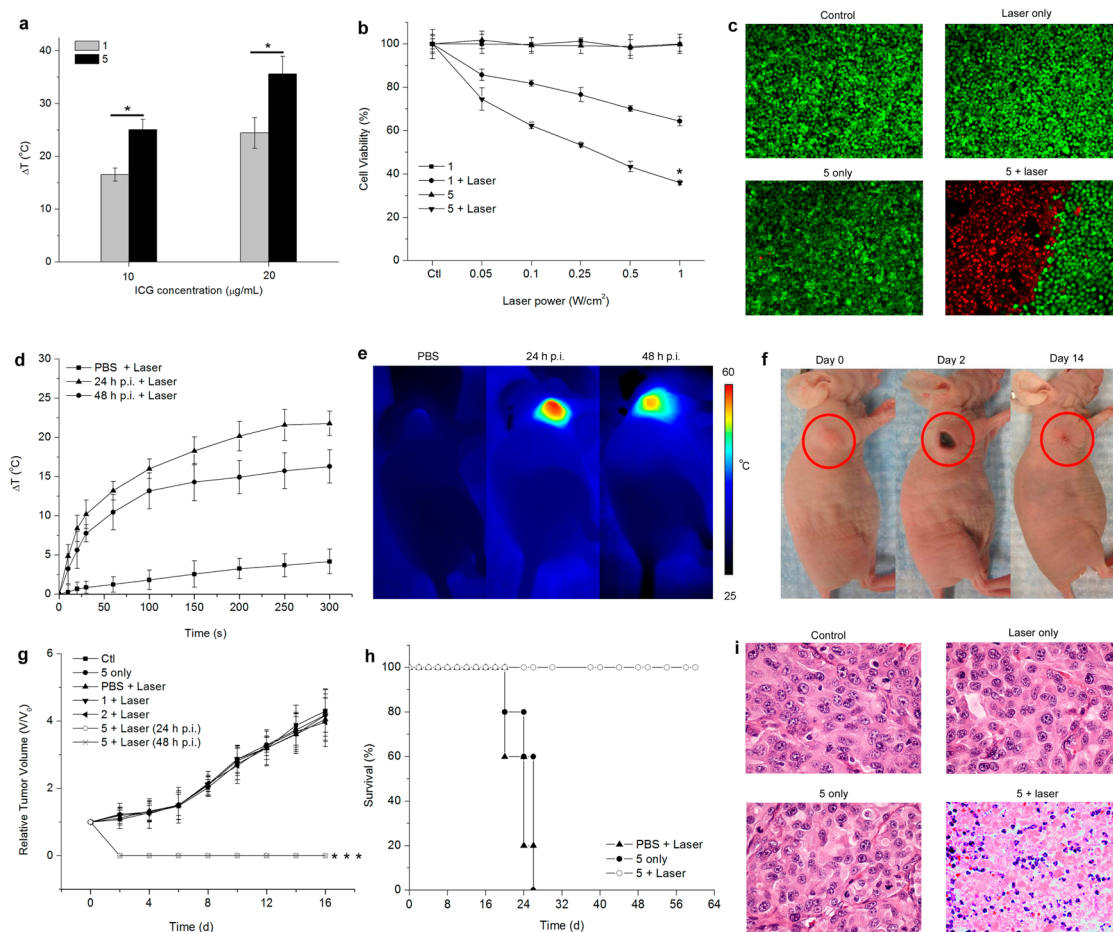
Figure 5. Photothermal effects of in situ enzyme-triggered self-assembly of 5 . (a) Heat generation ability of 1 and 5 in aqueous solutions ( 1 and 2 in a ratio of 1:100, 808 nm laser irradiation, 1 W/cm 2 , 3 min). * P < 0.05. (b) Relative viabilities of HeLa cells incubated with 1 (1, 10 μg/mL) and 5 (1, 10 μg/mL; 2 , 500 μg/mL) for 4 h with or without 808 nm laser irradiation (0.05–1 W/cm 2 , 3 min). * P < 0.05. (c) Calcein AM and PI costaining of HeLa cells incubated with 1 and 5 for 4 h with or without 808 nm laser irradiation (1 W/cm 2 , 5 min). (d) Heating curves of HeLa tumors upon laser irradiation as a function of irradiation time. (e) Thermal images of HeLa tumor-bearing mice at 24 and 48 h p.i. ( 1 at 5 mg/kg, and 2 at 100 mg/kg) with exposure to 808 nm laser irradiation (0.8 W/cm 2 , 5 min). (f) Photographs of HeLa-tumor-bearing mice at different days after PTT treatment. (g) Tumor growth curves of different groups of HeLa-tumor-bearing mice after PTT treatment. Tumor volumes have been normalized to their initial sizes. Error bars represent the standard deviations of five mice per group. *** P < 0.001. (h) Survival curves of the HeLa tumor mice after various treatments. (i) Hematoxylin and eosin staining of tumor sections collected from different groups of mice.
