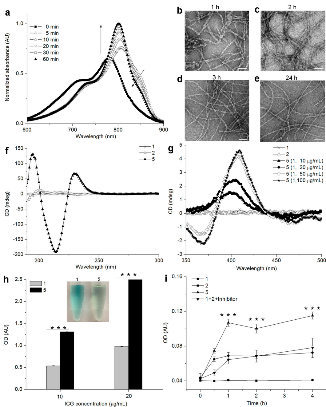
Figure 2. Optical property and structure conformations of 5. (a) Time-course UV-vis spectra of 5 during ALP-catalyzed process. (b–e) TEM images of 5 at different aging time points. (f) CD spectra of 1, 2, and 5. (g) CD spectra of 5 with different concentrations of 1 (2, 100 \mu\text{g/mL} ). (h) Optical density (OD) changes at 808 nm of 1 and 5 at different ICG concentrations (1 and 2 in a ratio of 1:100). The inset is the corresponding photograph of 1 at 10 \mu\text{g/mL} . *** P < 0.001 . (i) OD changes at 808 nm of cellular phosphatase-triggered self-assembly on HeLa cells incubated with different samples (1, 10 \mu\text{g/mL} ; 2, 500 \mu\text{g/mL} ). *** P < 0.001 .
