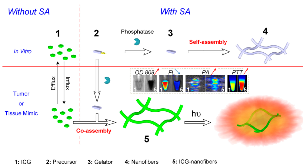
Scheme 1. Principle for enzyme-triggered supramolecular coassembly of 1 and 2 . In vitro : Precursor 2 is converted to hydrogelator 3 via dephosphorylation catalyzed by ALP. These hydrogelators self-assemble in water to form nanofibers 4 . Tumor or tissue mimic: 2 is catalyzed by a cellular phosphatase into 3 , which is able to coassemble with 1 and form ICG-doped nanofibers 5 . Within 5 , 1 takes the J -aggregate arrangement, which is evidenced by the red-shifted and significantly enhanced absorbance. 5 shows partially self-quenched fluorescence and enhanced photoacoustic and photothermal signals. However, without self-assembly, 1 is excreted shortly via efflux pump. Upon laser irradiation, 5 can efficiently convert photons into tumor-damaging heat.
